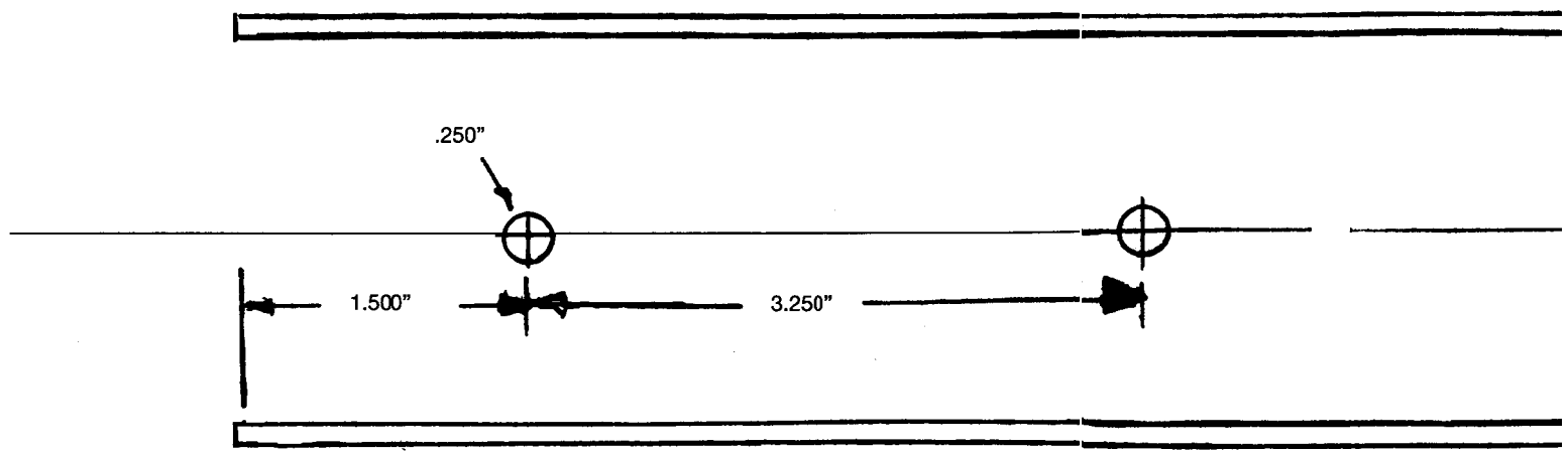
RECEIVER BOTTOM
