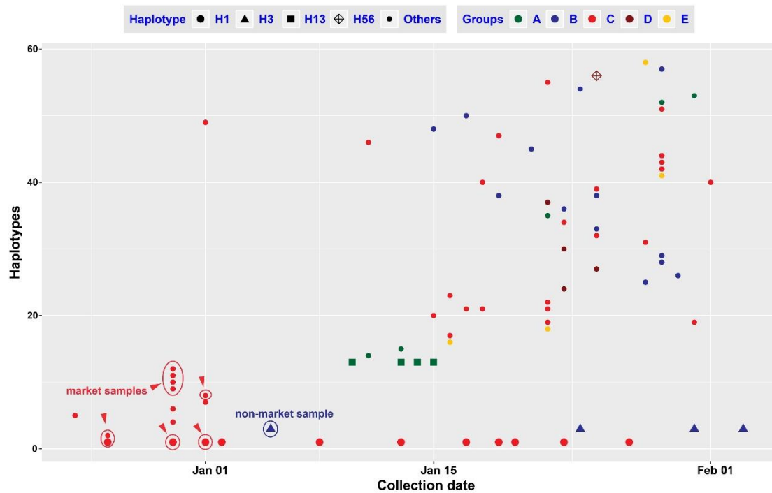
Figure 2. Genomic haplotypes of SARS-CoV-2 changes between the collection dates of samples. The confirmed samples from the Huanan Seafood Wholesale Market are indicated using red circles, and a confirmed sample with no link to the market is indicated using a blue circle.
