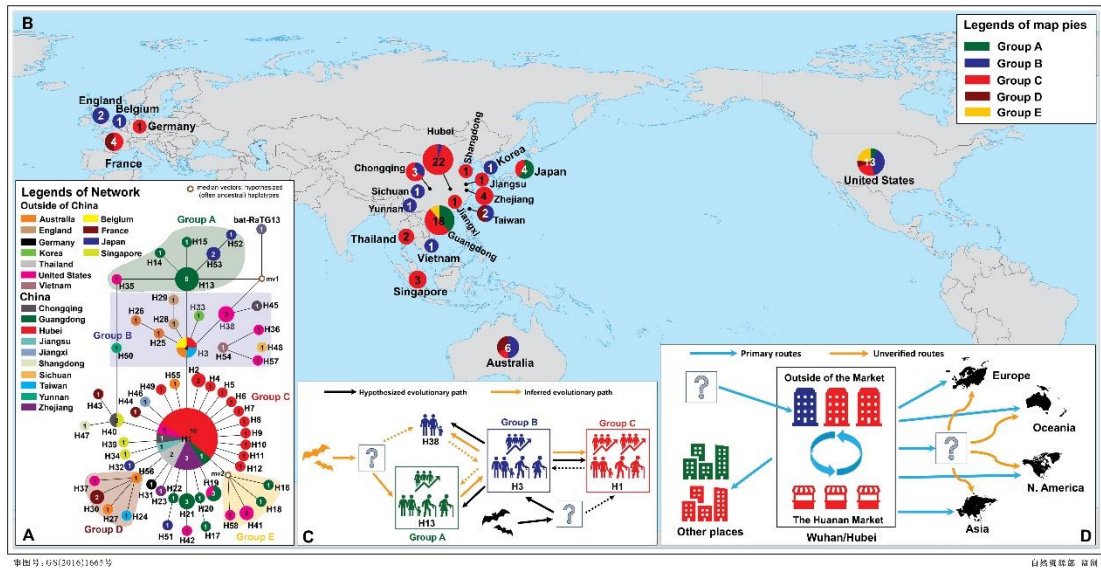
Figure 3. Evolutionary relationship and geographical distribution of 58 haplotypes of SARS-CoV-2 (A, B). Proposed evolutionary paths (C) of haplotypes and possible transmission and spreading routes (D) are also inferred based on evolutionary analyses and epidemiologic research. Sample sizes of haplotypes and regions are annotated in the circles.
