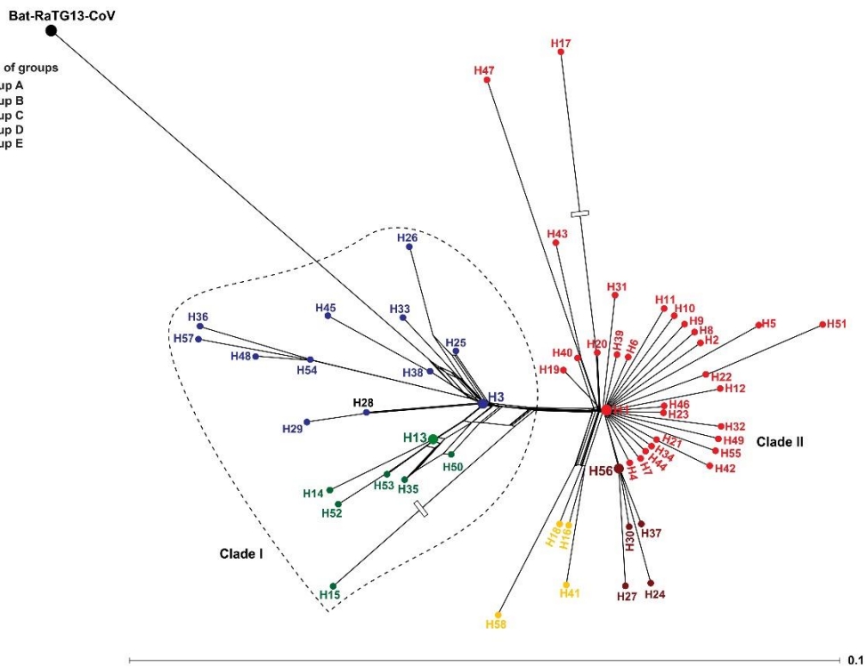
Figure 4. Phylogenetic networks of 58 haplotypes of SARS-CoV-2 with the outgroup bat-RaTG13-CoV using the whole coding region matrix (A) and 120 substitution sites (B), referring to all variable sites of coding regions in SARS-CoV-2 haplotypes. The bottom scale bars represent the number of substitutions per site. The open box on branches of bat-RaTG13-CoV (A), H15 (A, B), and H17 (A, B) indicating a long branch was clipped.
